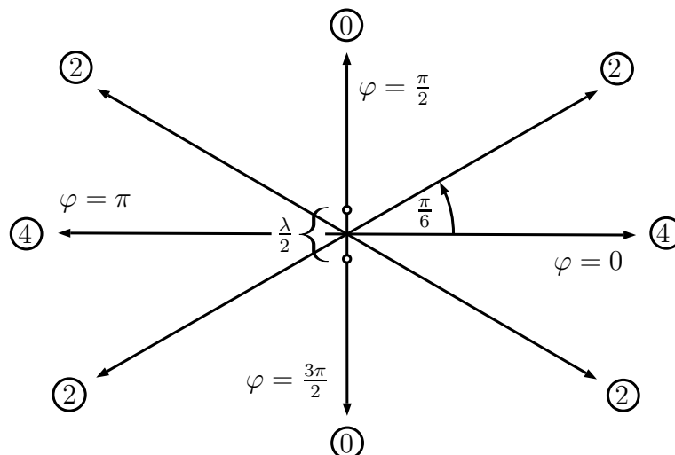
Abbildung 3.61: \phi_2 - \phi_1 = \pi \sin \varphi , I_2/I_1 = 4 \cos^2 \frac{\pi \sin \varphi}{2}
