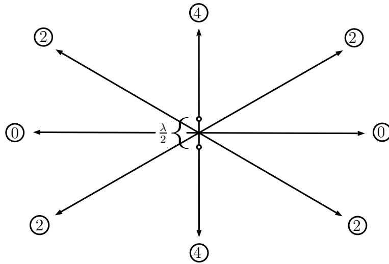
Abbildung 3.62: \phi_2 - \phi_1 = \pi \sin \varphi + \pi , I_2/I_1 = 4 \cos^2 \frac{\pi(\sin \varphi + 1)}{2}
