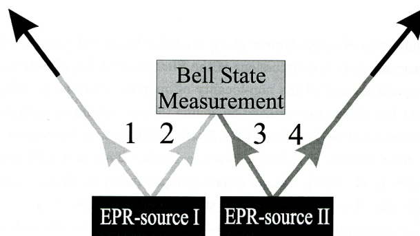
Figure 4.1: Principle of entanglement swapping. Two EPR sources produce two pairs of entangled photons, pair 1-2 and pair 3-4. One photon from each pair (photon 2 and 3) is subjected to a Bell-state measurement (BSM). This results in projecting the other two outgoing photons 1 and 4 into an entangled state. Change of the shading of the lines indicates a change in the set of possible predictions that can be made.
